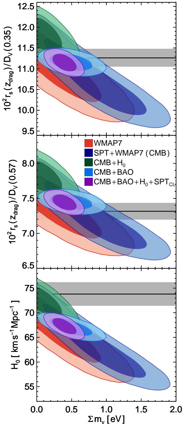
FIG. 8.— This figure shows how low-redshift datasets affect the neutrino mass constraints. In the planes of \sum m_\nu and three quantities inferred at low redshifts, we show the marginalized two-dimensional posteriors from different combinations of datasets shown by the legend in the central panel. Top : constraints are plotted in the \sum m_\nu - r_s(z_{\text{drag}})/D_V(0.35) plane with the SDSS BAO data point shown by the grey band as the 1\sigma region. Middle : similar to the left panel but showing r_s(z_{\text{drag}})/D_V(0.57) with the BOSS BAO data point shown by the grey band as the 1\sigma region. Bottom : similar to the top and middle panels but showing H_0 with the grey band showing the 1\sigma region. The tension between BAO and H_0 can be seen in the three panels. The CMB+BAO preference for massive neutrinos is clearly visible.
