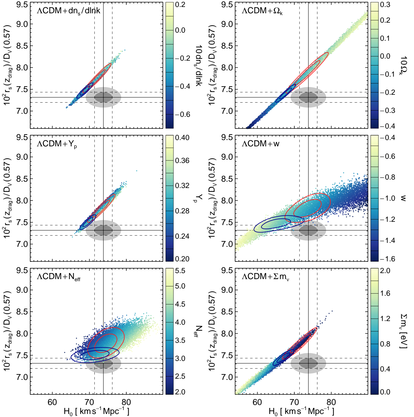
FIG. 3.— This figure expands Figure 2 to investigate the consistency between the CMB, \text{BAO}_{\text{BOSS}} , and H_0 datasets in one-parameter extensions to \Lambda\text{CDM} . Each panel shows the H_0 - r_s/D_V(0.57) plane for a different extension. The colored dots are samples drawn from the SPT+ WMAP7 MCMC chain, with the color coding reflecting the value of the extension parameter, as shown in the color scales on the right. The horizontal solid and dashed lines mark the central value and 1\sigma region for the \text{BAO}_{\text{BOSS}} measurement, while the vertical lines do the same for H_0 . The joint 1 and 2\sigma likelihood region for \text{BAO}_{\text{BOSS}}+H_0 measurements is denoted by the dark and light grey shaded contours. The blue (red) contours overlaid show the 68\% and 95\% confidence regions for CMB+BAO (CMB+ H_0 ). Varying the effective number of neutrino species leads to the best agreement between the CMB, \text{BAO}_{\text{BOSS}} , and H_0 .
