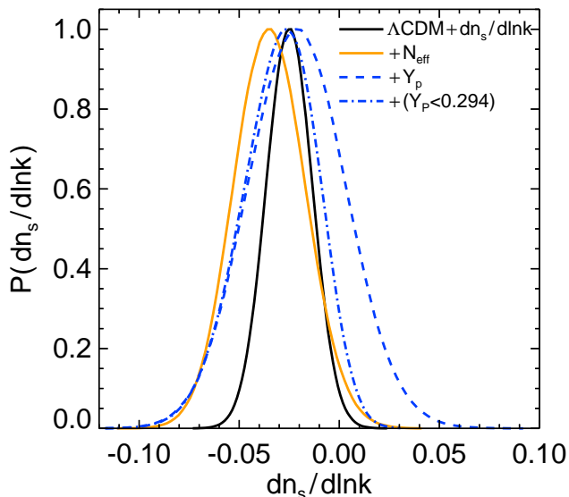
FIG. 12.— The preference of the SPT + WMAP7 data for negative running remains as additional parameters are freed. The marginalized one-dimensional posteriors for dn_s/d\ln k from the CMB in the \Lambda\text{CDM}+dn_s/d\ln k model is shown by the black solid line. The preference for negative running is reduced when Y_p is allowed to vary (blue dashed line), although this depends on extremely high helium abundances. If an upper limit based on solar abundances is set on Y_p , the preference for negative running is mostly restored (blue dot-dashed line). Allowing N_{\text{eff}} to vary (orange solid line) increases the preference for negative running.
