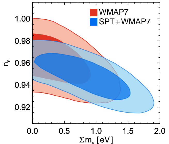
FIG. 6.— This figure illustrates the degeneracy between n_s and \sum m_\nu , and its role in the SPT+ WMAP7 preference for nonzero neutrino masses. The contours are the 68% and 95% confidence intervals in the \Lambda CDM+ \sum m_\nu parameter space for WMAP7 (red) and SPT+ WMAP7 (blue). The SPT data prefer a lower value of n_s than WMAP7 , which leads the CMB data to prefer higher \sum m_\nu .
