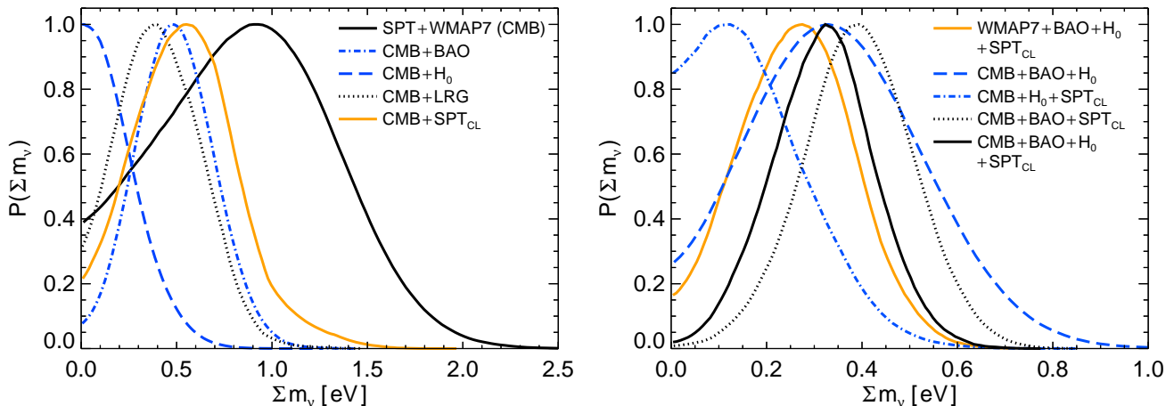
FIG. 9.— Left panel: This panel demonstrates how the marginalized one-dimensional posterior distribution of \sum m_\nu changes when a single external dataset is added to the CMB dataset. The CMB constraint is shown by the black solid line. The datasets added are the BAO data (blue dot-dashed line), H_0 measurement (blue dashed line), LRG sample (black dotted line), and SPT cluster data (orange solid line). Right panel: This panel demonstrates how the marginalized one-dimensional posterior distribution of \sum m_\nu changes when a single external dataset is removed from the combination of CMB+BAO+ H_0 +SPT CL . The datasets dropped are the SPT bandpowers (orange solid line), SPT CL (blue dashed line), BAO data (blue dot-dashed line), and H_0 measurement (black dotted line). The marginalized posterior for the combined CMB+BAO+ H_0 +SPT CL dataset is shown by the black solid line.
